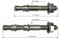
Art. 121 Hang Fix Ø 8 mm Art. 122 inox
